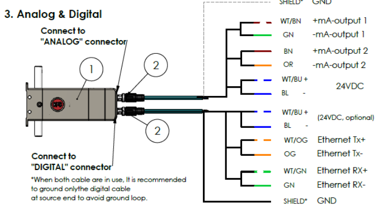
Figure 2 Inline concentration monitor DCM-10 operation concept. DWG No. 10125.
