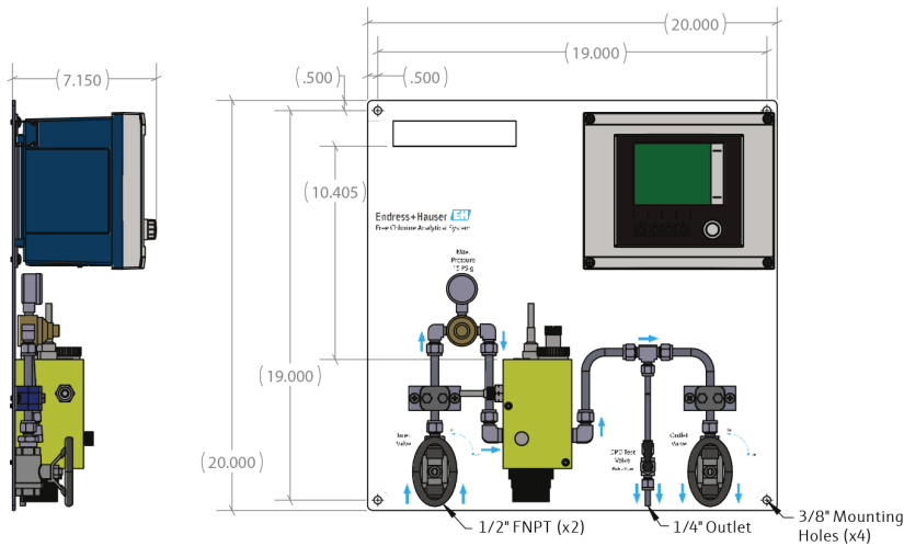
Free and total chlorine disinfection measurement systems
