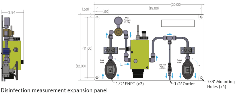
Disinfection measurement expansion panel
